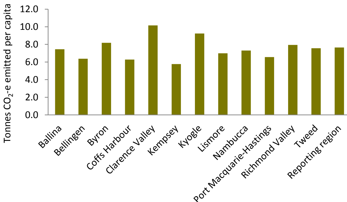
Figure 9: Tonnes CO 2 -e emitted per person from electricity consumption for 2011-12 (Source: Essential Energy)
