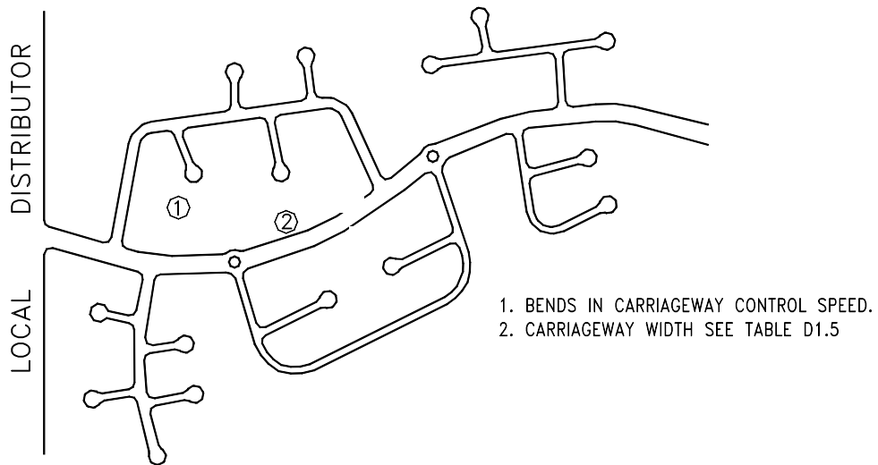
Figure D1.5 Collector Road
