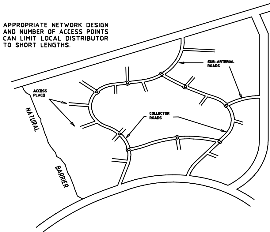
Figure D1.6 Sub-Arterial Road
